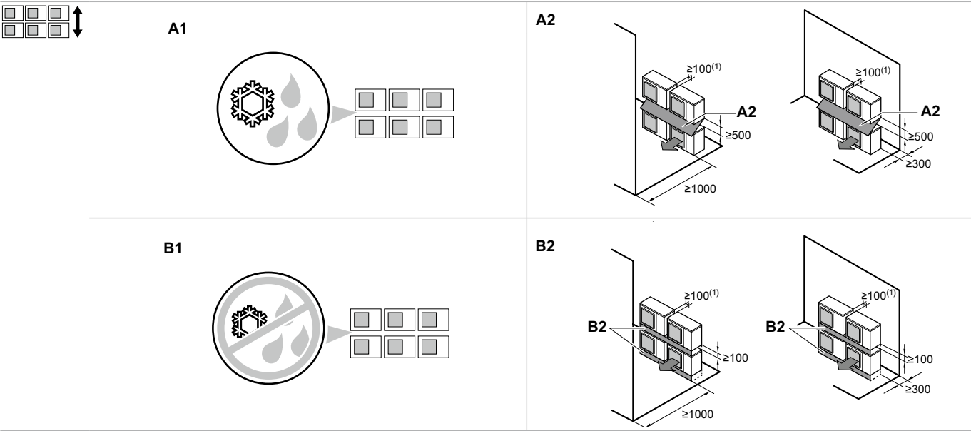
(1) For better serviceability, use a distance \geq 250 mm A1=>A2 (A1) If there is danger of drainage dripping and freezing between the upper and lower units... (A2) Then install a roof between the upper and lower units. Install the upper unit high enough above the lower unit to prevent ice buildup at the upper unit's bottom plate. B1=>B2 (B1) If there is no danger of drainage dripping and freezing between the upper and lower units... (B2) Then it is not required to install a roof, but seal the gap between the upper and lower units to prevent discharged air from flowing back to the suction side through the bottom of the unit.
