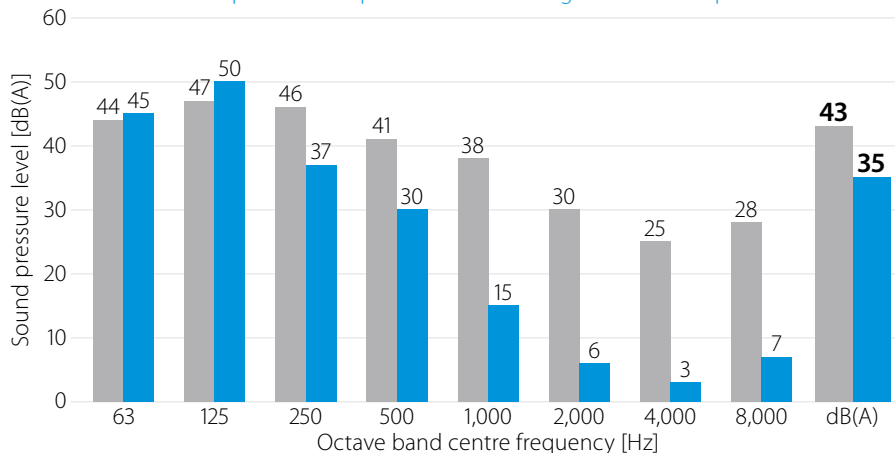
Example of sound pressure level cooling in low noise operation
