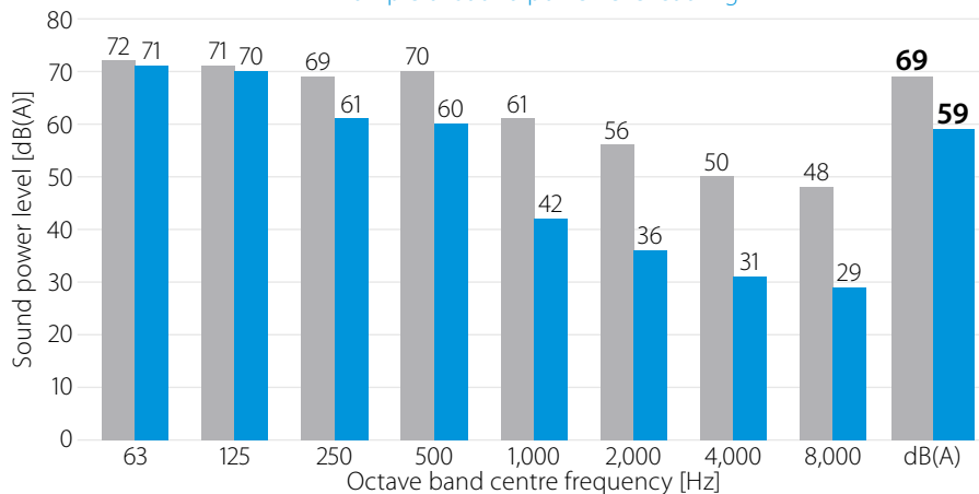
Example of sound pressure level cooling
